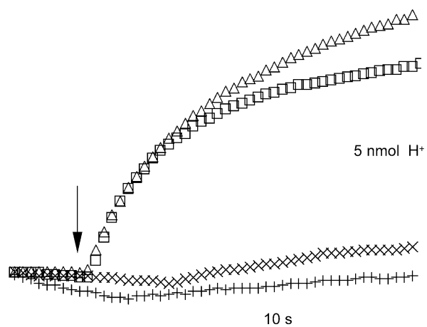
Fig. 2. Proton uptake in the proteoliposomes containing subunit a purified in chloroform-methanol-water mixture after reconstitution with subunits b and c . Proteoliposomes with subunit c only (×), subunits a and b only (+), subunits a , b and c (Δ), or purified complete F_0 complex (□).
